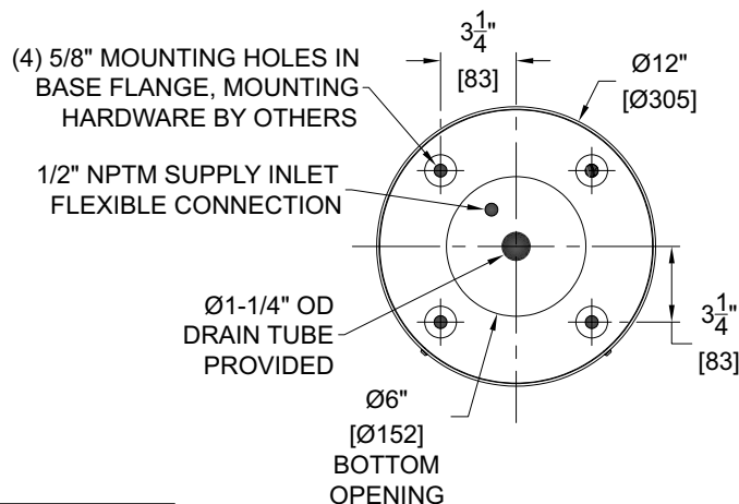
BASE FLANGE MOUNTING DETAIL
