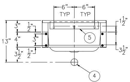
ROUGH-IN-DIMENSIONS
